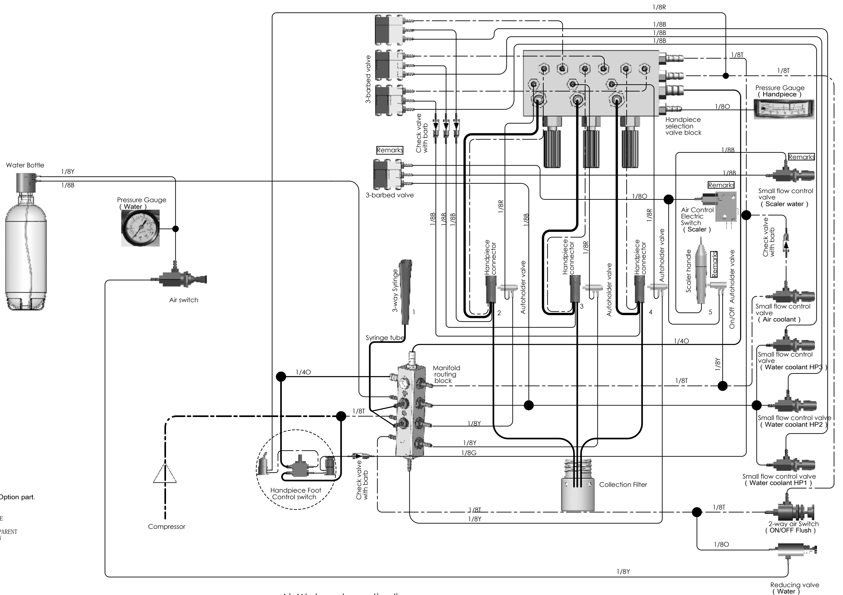
Air Water schematic diagram
